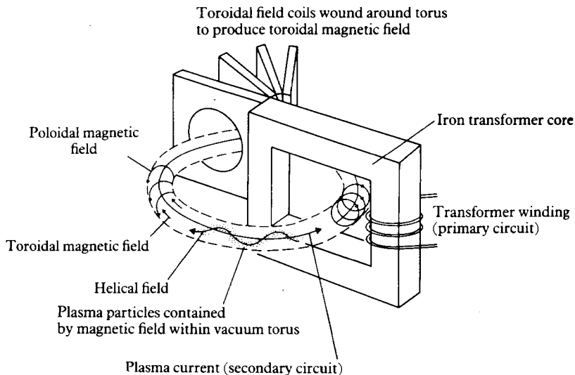
14.12 A schematic diagram of a Tokamak machine.
